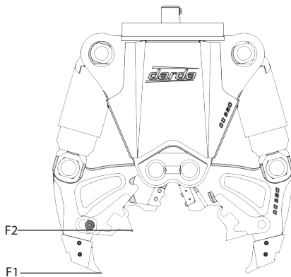
Additional crusher tips
